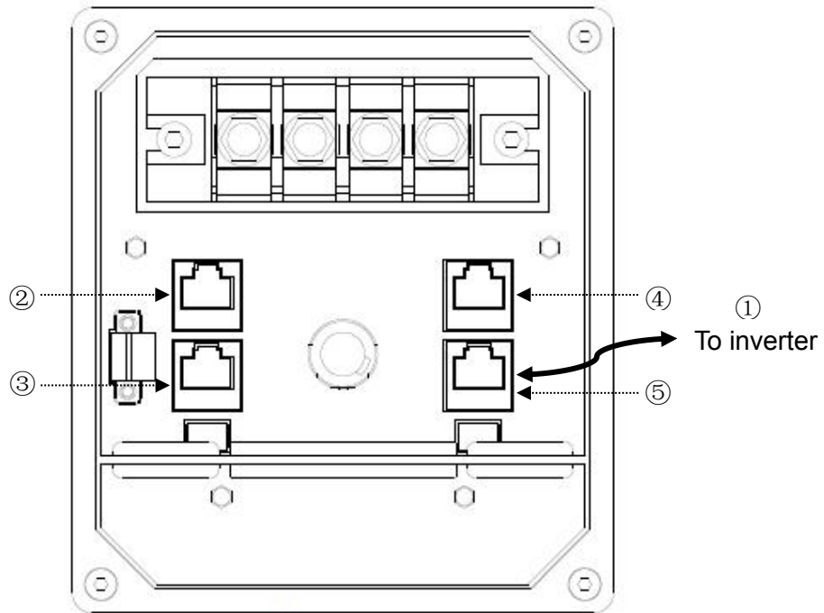
Figure 3.3 CAN communication wiring
