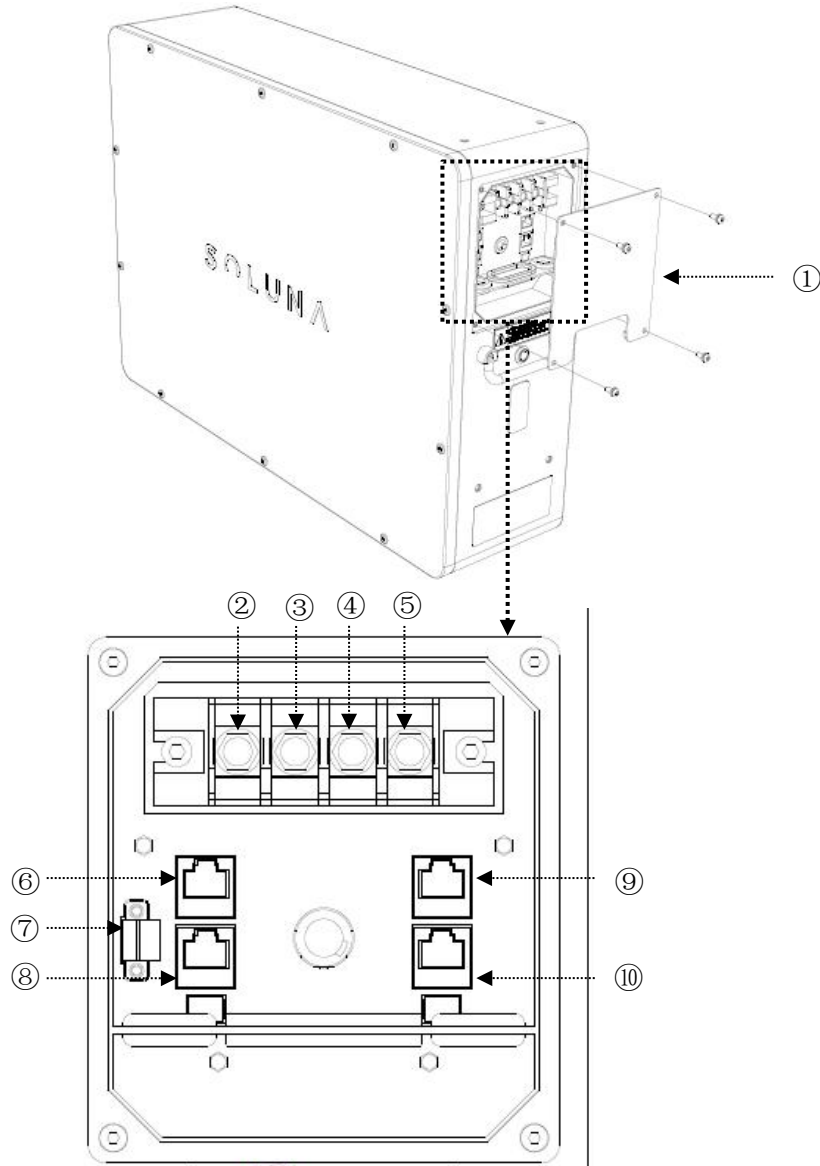
Figure 2.3 wiring port
