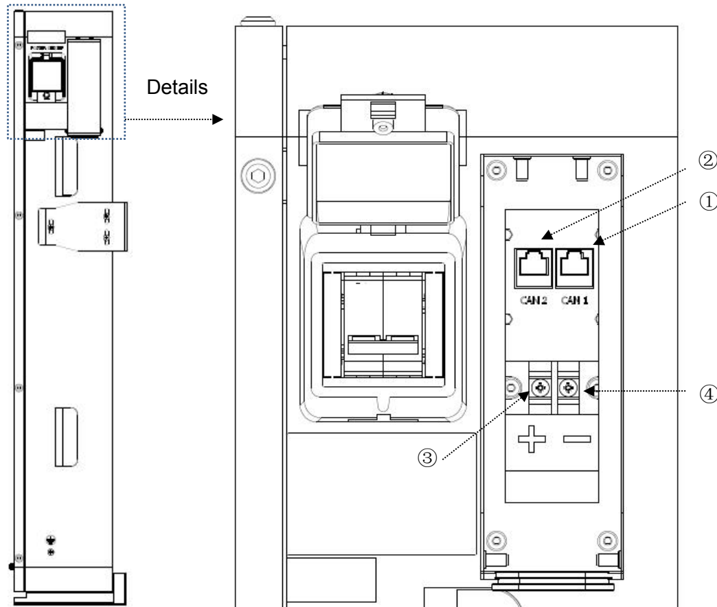
Figure 2.3 wiring port
