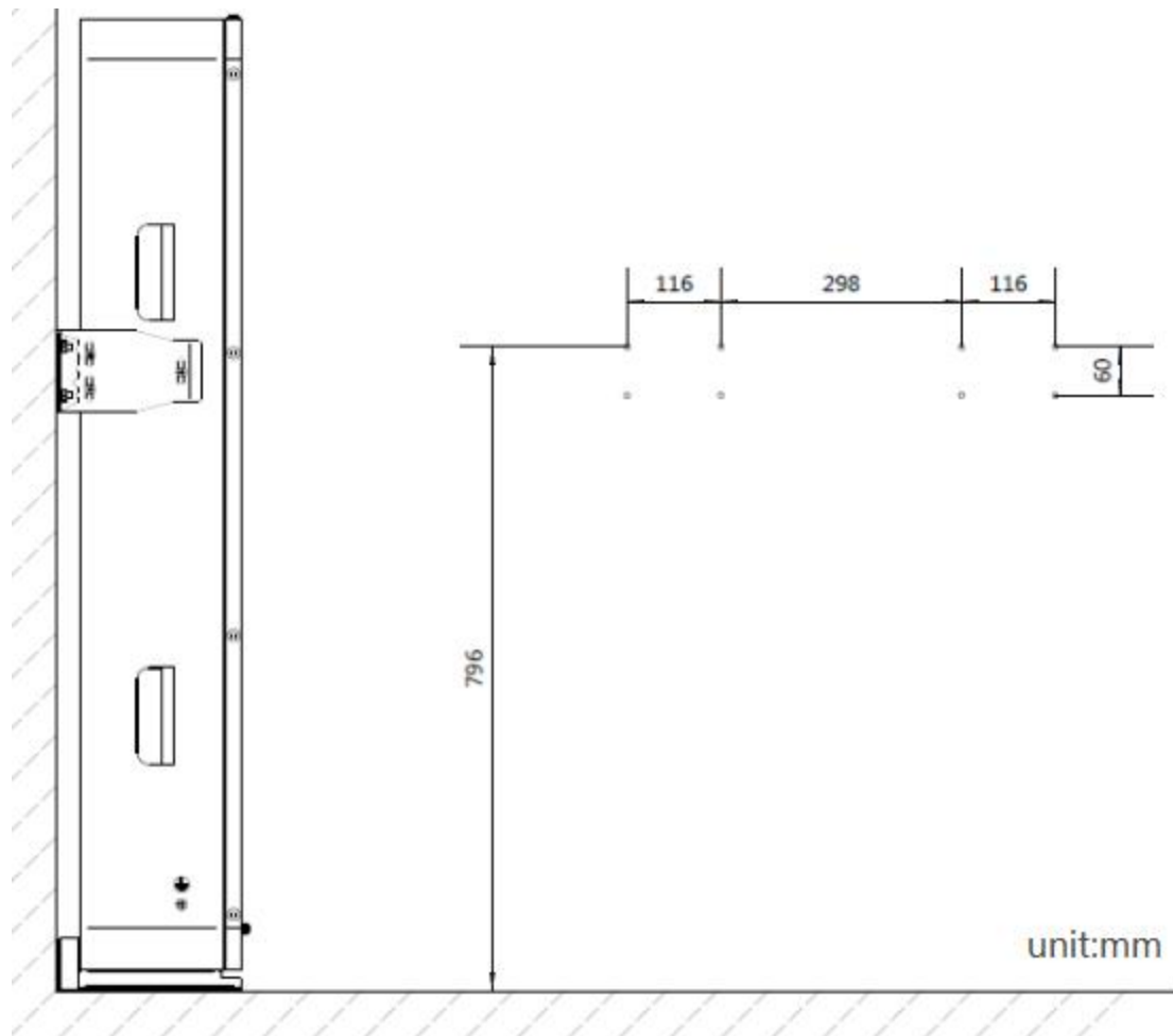
Figure 3.3 Installation requirement
